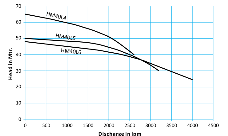
Performance Curves • Model : 40 HP
