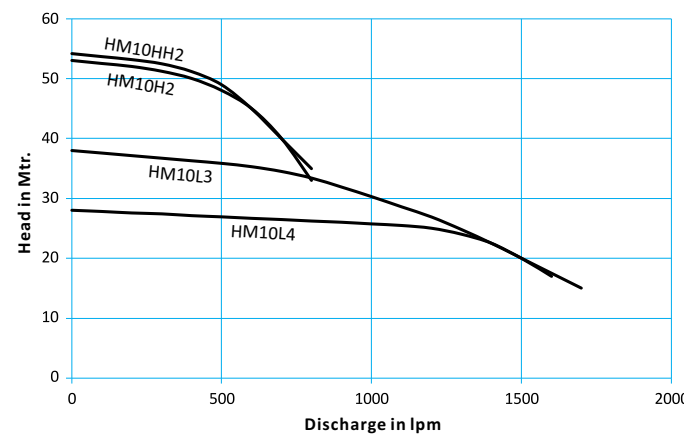
Performance Curves • Model : 10 HP
