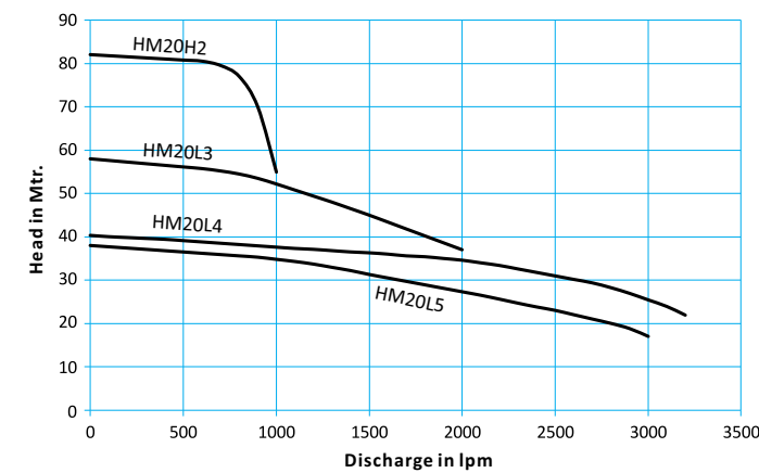
Performance Curves • Model : 20 HP
