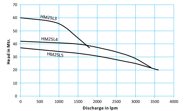
Performance Curves • Model : 25 HP
